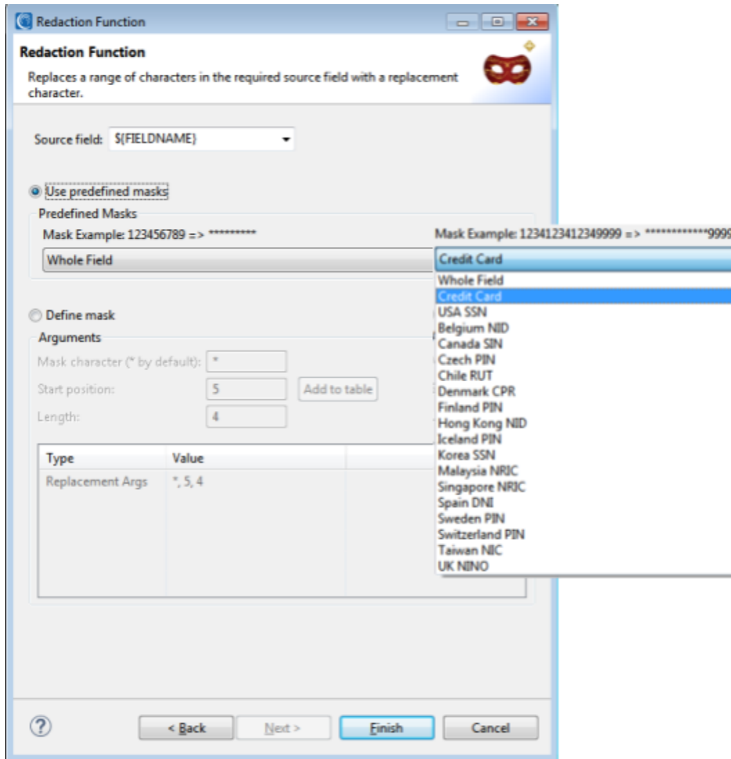
Data Redaction function dialog in the IRI Workbench IDE for FieldShield, DarkShield, etc, built on Eclipse™
