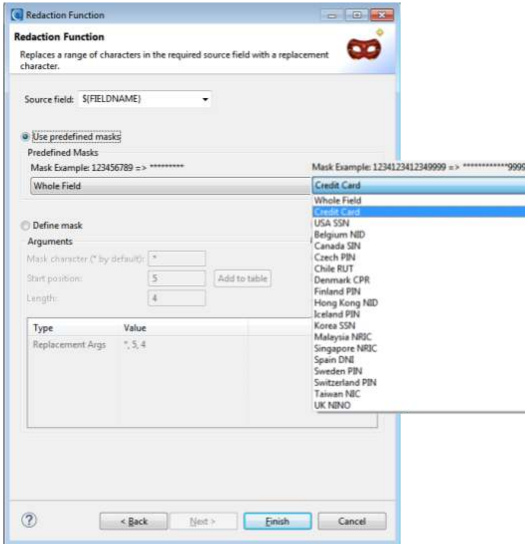
Data Redaction function dialog in the IRI Workbench IDE for FieldShield, Voracity, etc., built on Eclipse™
